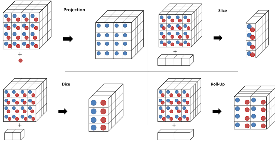
Fig. 3. Illustration of common OLAP operations with inputs and outputs (adapted from [21])
