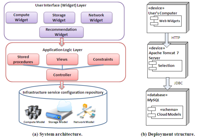
FIGURE 3: CLOUDRECOMMENDER SYSTEM ARCHITECTURE.
