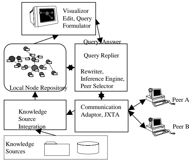
Figure 1. The SWAP architecture.
