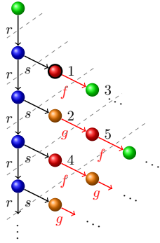
Figure 3: An initial collapsing for the unravelling depicted in Figure 2.
