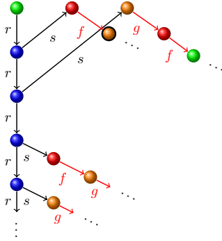
Figure 5: A collapsing obtained from the one depicted in Figure 4.
