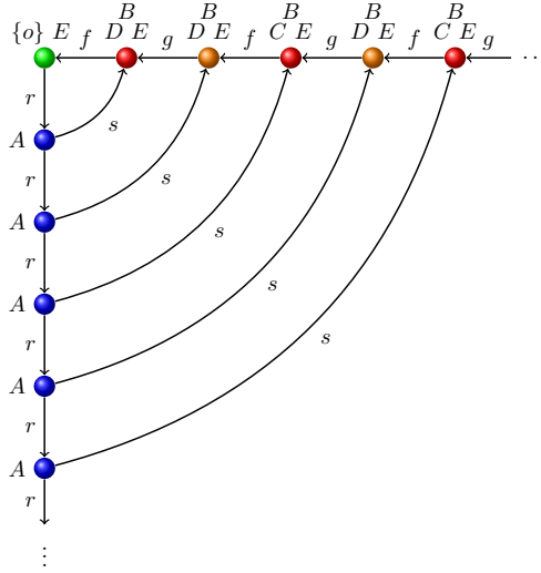
Figure 7: Result of collapsing the unravelling from Fig. 2. The infinitely many new root elements are displayed in the top line.
