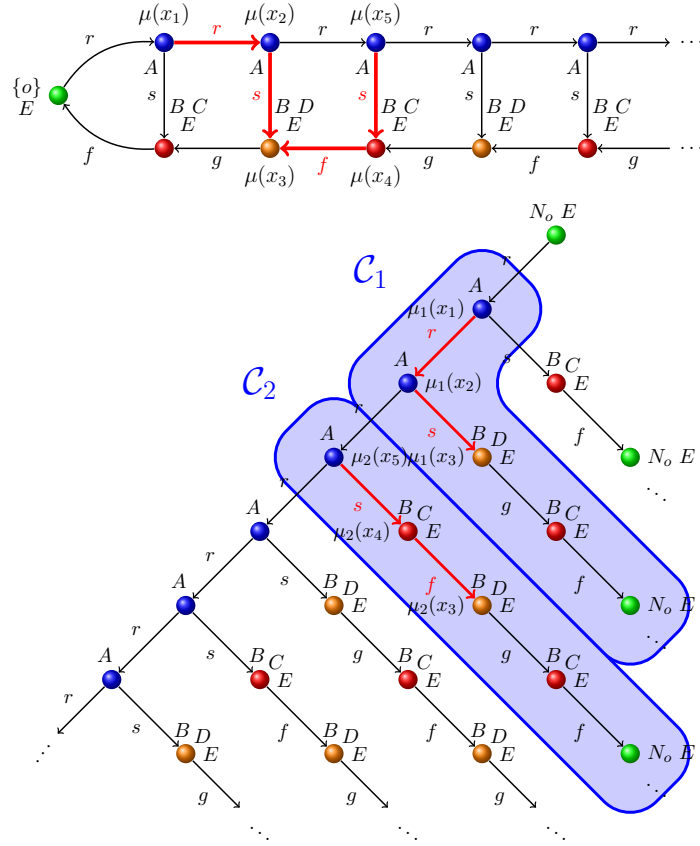
Figure 8: Correspondence between entailment and quantailment.
