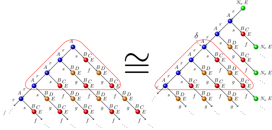
Figure 10: Forest quasi-model (right) and according 3-secure replacement for \delta (left).
