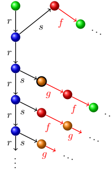
Figure 4: In the first collapsing step we just rename elements to promote the focus from Figure 3 to a root.
