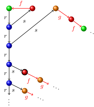
Figure 6: A collapsing obtained by using the second case of Definition 17 on the collapsing from Figure 5.
