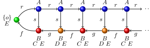
Figure 1: Knowledge base and model.
