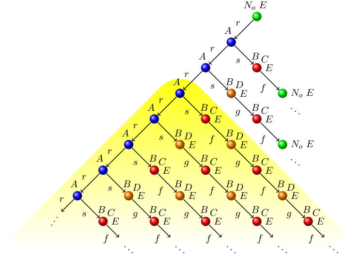
Figure 11: Result of replacing the element \delta by the 3-secure replacement depicted in Figure 10. The inserted component is highlighted.
