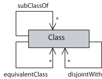
Figure 4: Class axioms
