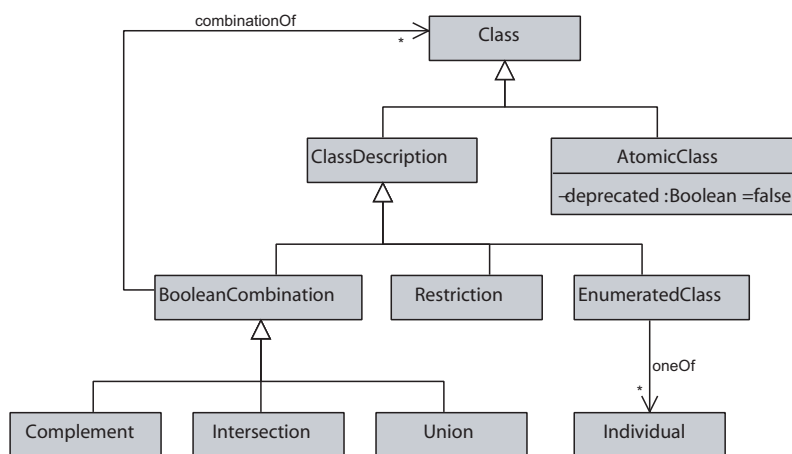
Figure 3: Class constructors
