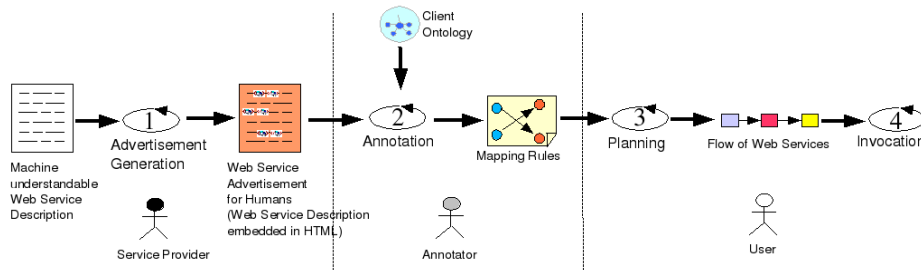
Fig. 7. The Complete Process of OntoMat-Service
