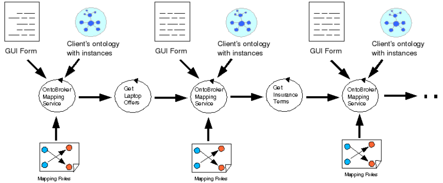
Fig. 12. Service Flow in our Running Example
