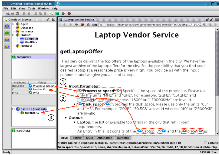
Fig. 9. Screenshot of OntoMat-Service-Surfer annotating vendor service
