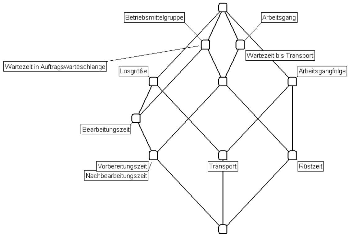
Figure 2: The concept lattice of the formal context in Fig. 1
