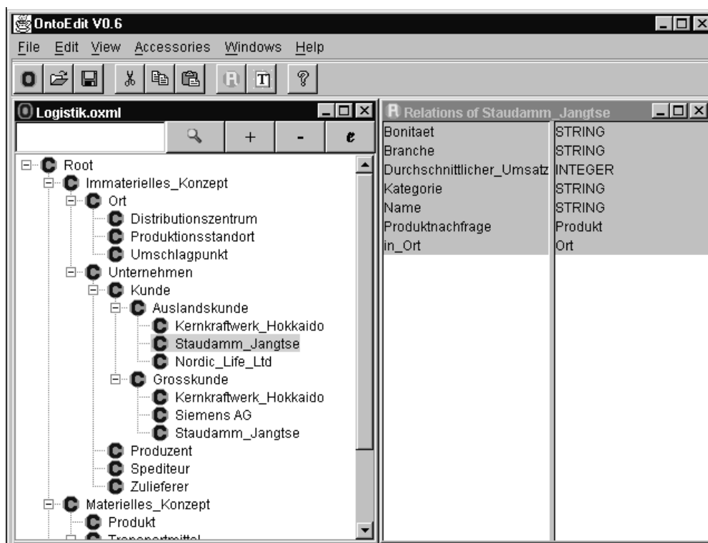
Figure 3: An ontology about logistics
