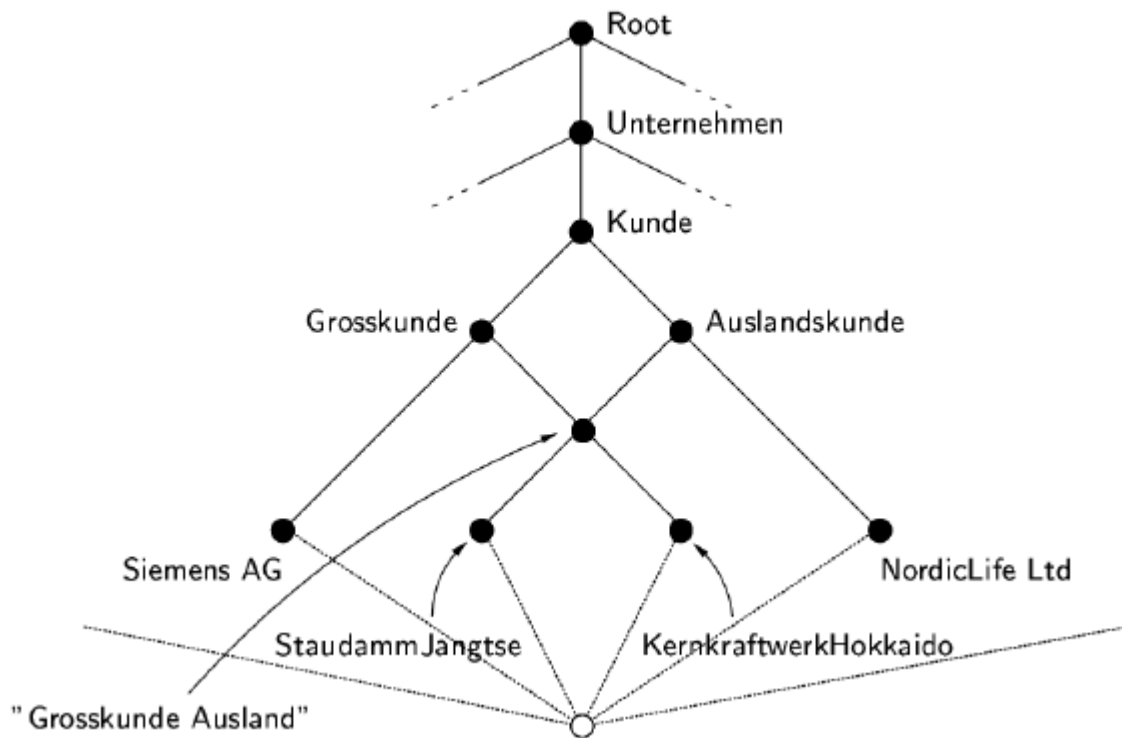
Figure 5: Dedekind-MacNeille-completion of the "customer" part. (The new bottom concept arises out of theoretical reasons and can be ignored in practice.)
