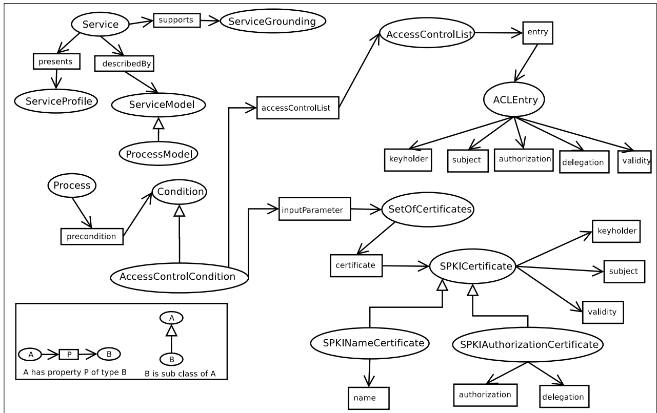
Figure 1: Integration of DAML-S and SPKI
